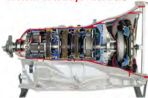
MEGART1282 6 Gear Automatic Transmission
